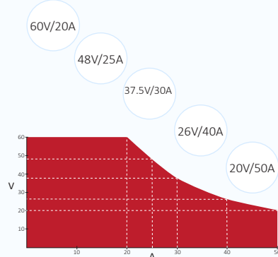
QPX1200S/SP PowerFlex
