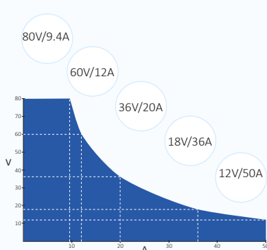
QPX750SP PowerFlex+
