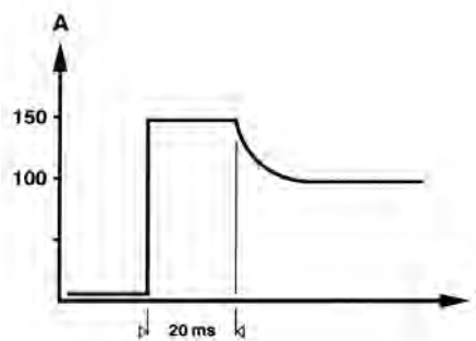
Brief load current with TOE 8872-40 (TOE 8871/022 option)
